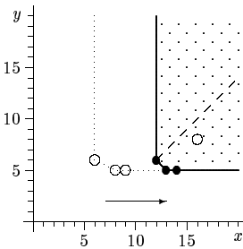
FIGURE 6 The polyhedron N(A^3)
