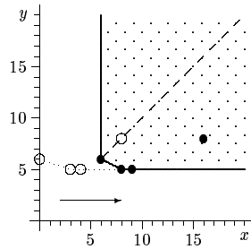
FIGURE 5 The polyhedron N(A^2)
