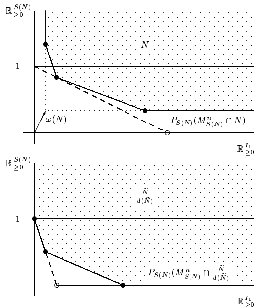
FIGURE 8 Illustration of Spivakovsky's notation
