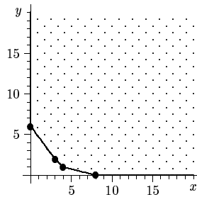
FIGURE 3 The polyhedron N(A)
